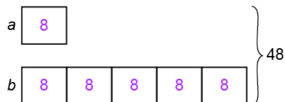
Figure 18: using a bar model to solve a problem with 2 unknowns – example 2
