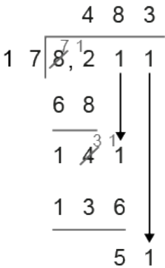
Figure 37: long division calculation ( 8,211 \div 17 )
