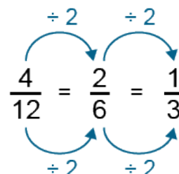
Figure 22: simplifying \frac{4}{12} in 2 steps
