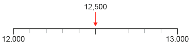
Figure 3: placing 12,500 on a 12,000 to 13,000 number line marked, but not labelled, in multiples of 100
