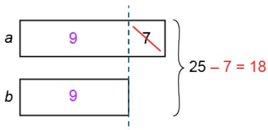
Figure 17: using a bar model to solve a problem with 2 unknowns – example 1
