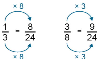
Figure 26: expressing \frac{1}{3} and \frac{3}{8} in twenty-fourths
