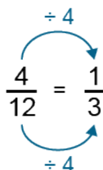
Figure 21: simplifying \frac{4}{12} by dividing the numerator and denominator by the highest common factor
