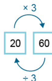
Figure 12: multiplicative relationship between 20 and 60
