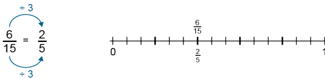
Figure 20: simplifying \frac{6}{15} by dividing the numerator and denominator by the common factor of 3
