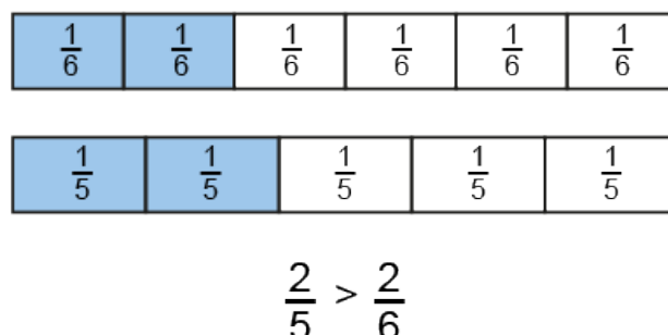
Figure 27: bar models to compare \frac{2}{5} and \frac{2}{6}
