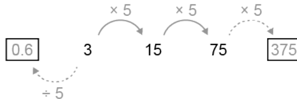
Figure 14: completing a sequence where each term is 5 times the previous
