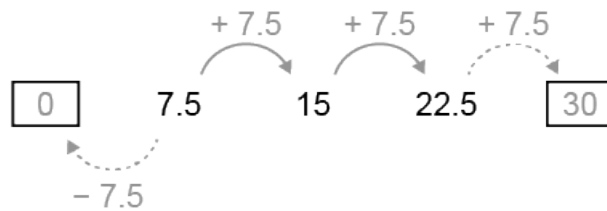
Figure 13: completing a sequence where the difference between adjacent terms is 7.5
